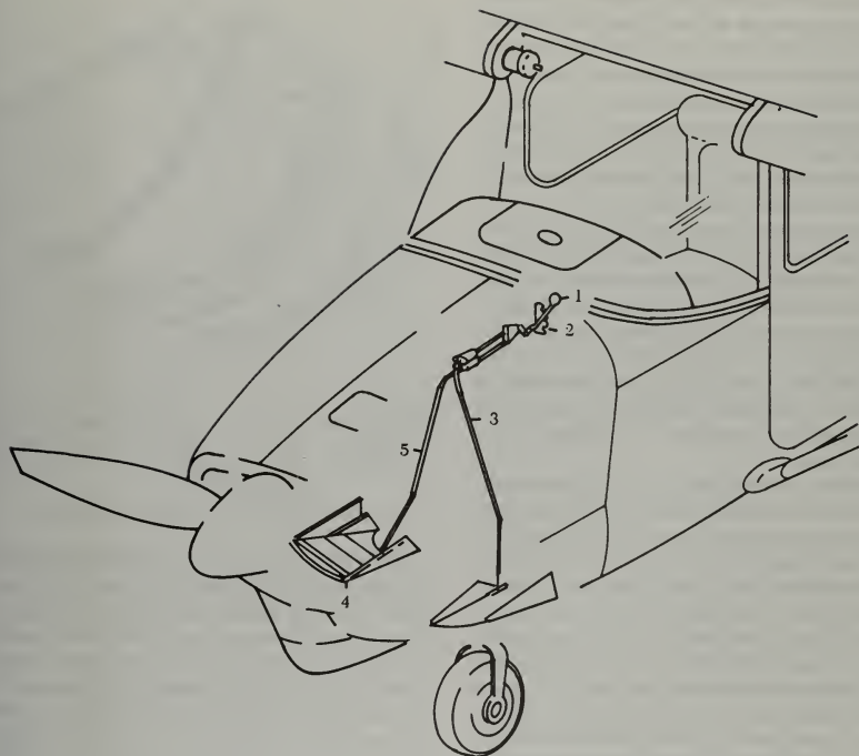
FIGURE 6-38. Small aircraft cowl flaps.
